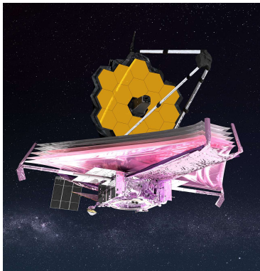
James Webb - Hubble
